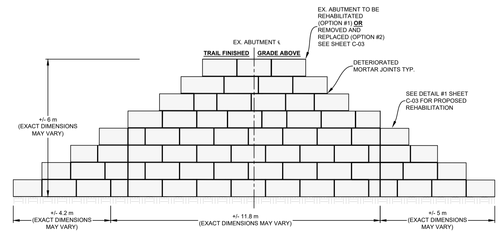
3 EXISTING WEST ABUTMENT SCALE: 1:100
