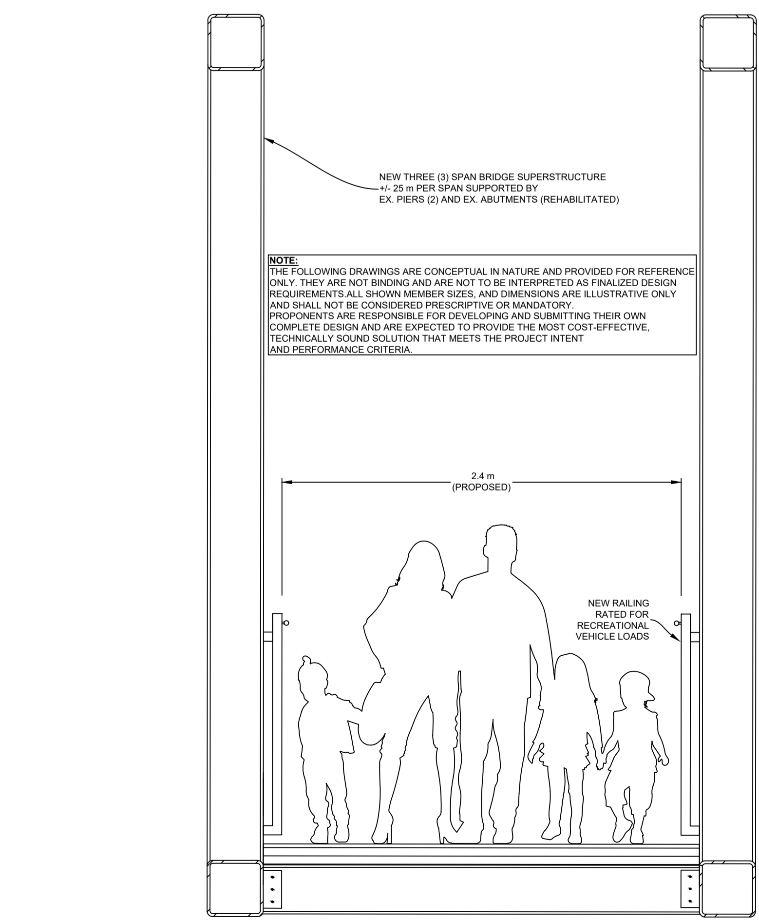
3 CONCEPTUAL BRIDGE SECTION (OPTION #1) SCALE: 1:20
